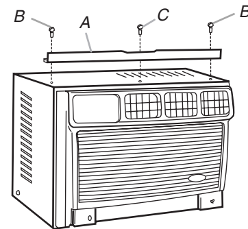
A. Top channel B. #10 x \frac{3}{8} " pan-head screw (on all models) C. #10 x \frac{3}{8} " pan-head screw (on some models)
